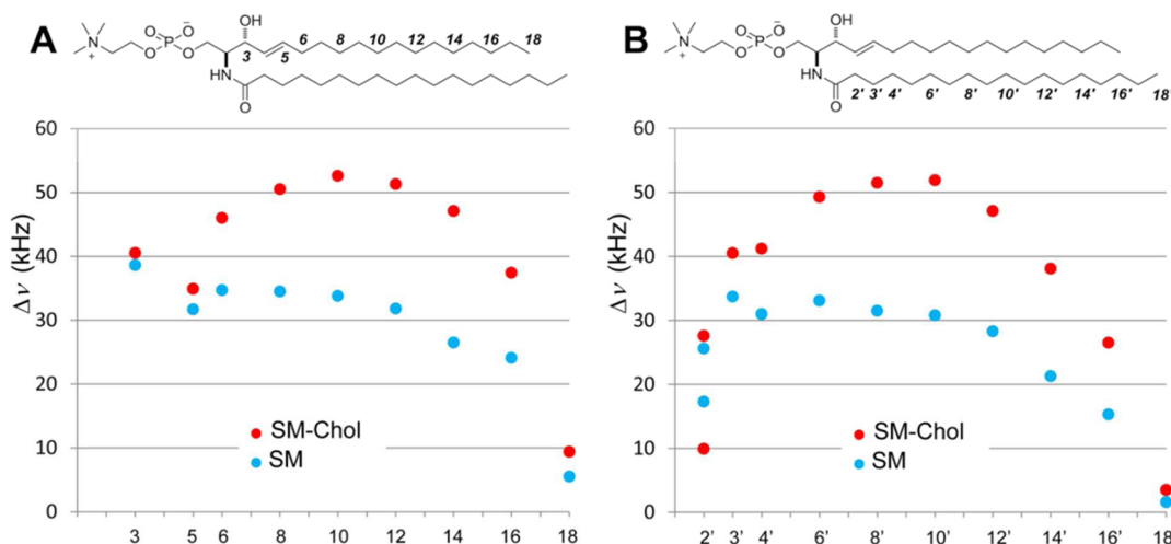
Figure 2. Quadrupole splitting profiles obtained from SSM that has been site-specifically deuterium-labeled on the sphingosine (A) and stearyl (B) chains. Data were obtained in the absence (blue circles) and presence (red ones) of 50 mol % Chol at 45 °C.
